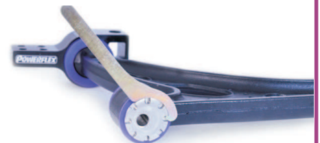
Maximum camber towards middle of car
