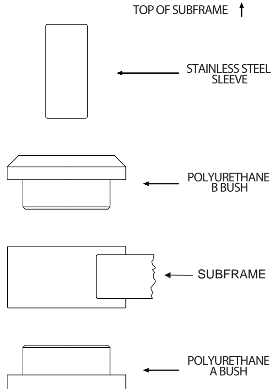
Figure 1: Assembly exploded view
