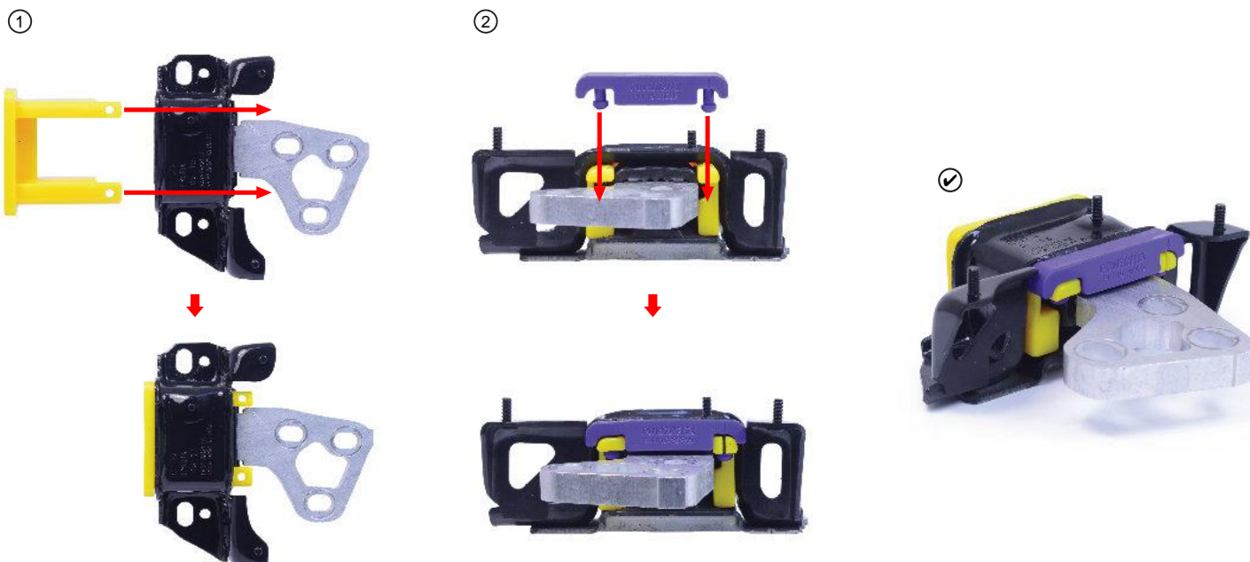
Figure 1: Fitted Assembly Steps
